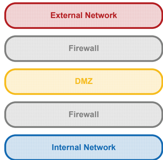
Figure 1: Network Security
